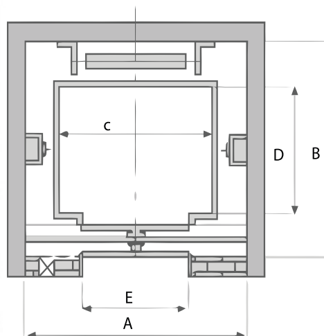
HOISTWAY ELEVATION PLAN
