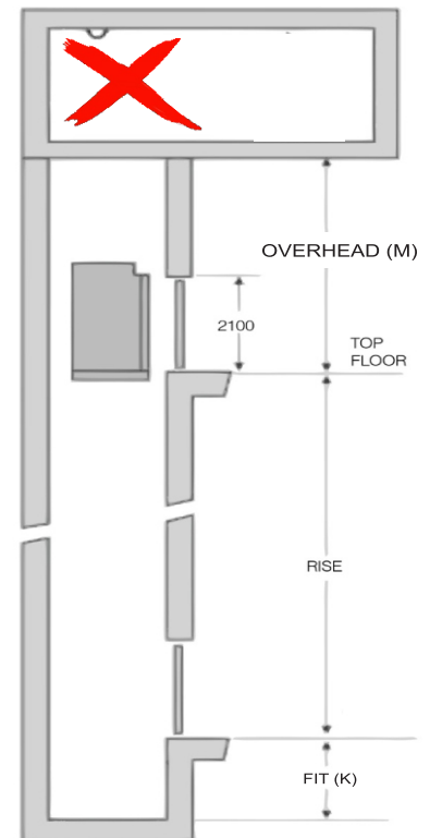
HOISTWAY ELEVATION DRAWING
