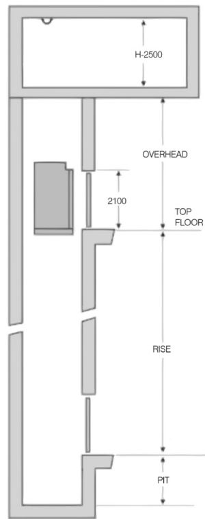
HOISTWAY ELEVATION PLAN
