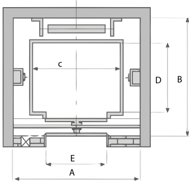
HOISTWAY ELEVATION PLAN
